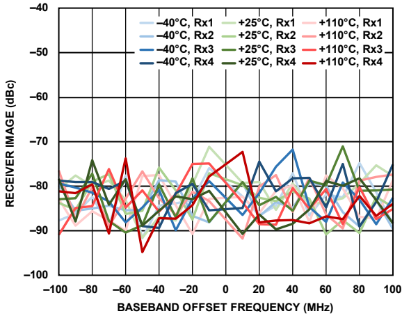
Figure 454. Receiver Image vs. Baseband Offset Frequency, Tracking Calibration Active, Sample Rate = 245.76 MSPS
