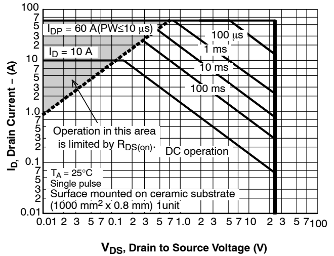
Figure 12. S O A
