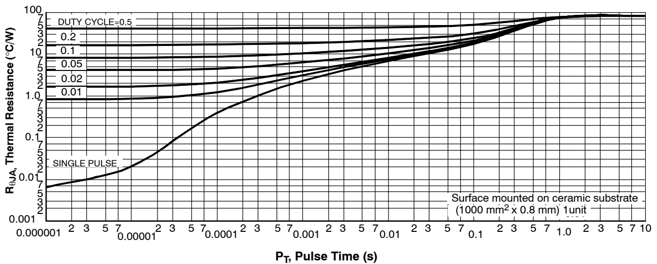
Figure 13. R_{\theta JA} - P_{T, Pulse Time}
