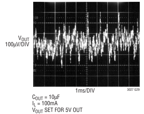
10Hz to 100kHz Output Noise C_{\text{BYP}} = 100\text{pF}
