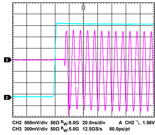
Figure 40. Enable Time Domain Response at V_{POS} = 3.3V
