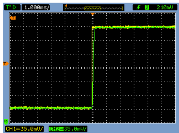
Figure 6: TS1005 Transient Response for R ISO = 50kΩ and C LOAD = 500pF.
