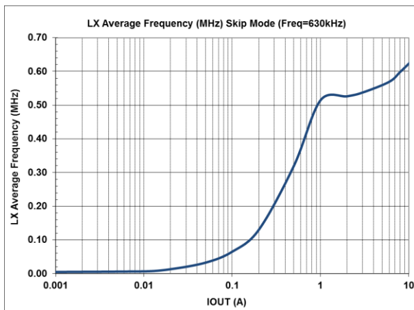
Frequency = 630 kHz
