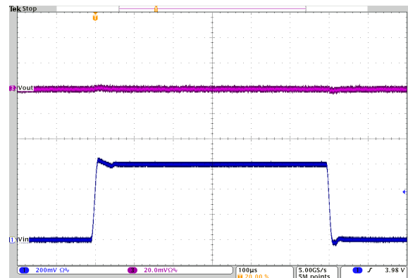
Figure 4-34. Line Transient Response LDO2
