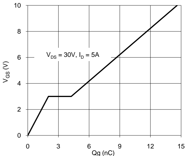
Figure 11. Gate Charge
