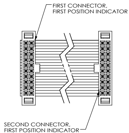
(FFSD-10-D-XX.XX-01-X-N-RN2 SHOWN) (SAME AS FIG 1, DIFFERENT AS SHOWN)
