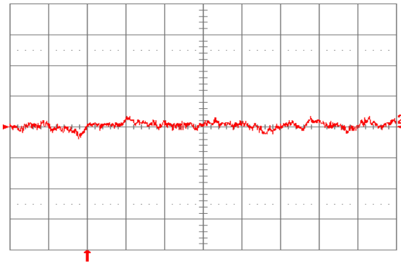
Figure 20. Input reflected ripple current, i_s (10 mA/div), measured through 10 \mu H at the source at full rated load current and V_{in} = 48 V. Refer to Fig. 19 for test setup. Time scale: 1 \mu s/div.
