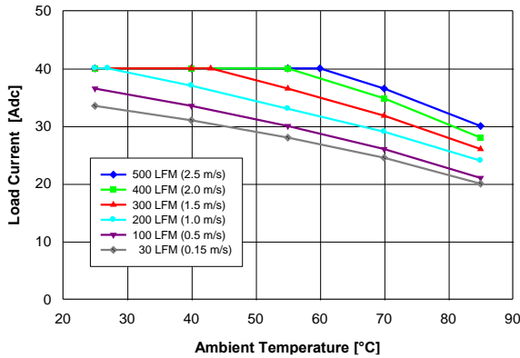
Figure 9. Available load current vs. ambient air temperature and airflow rates for QM48S40033 converter mounted vertically with air flowing from pin 3 to pin 1, MOSFET temperature \leq 120 °C, V_{in} = 48 V.
