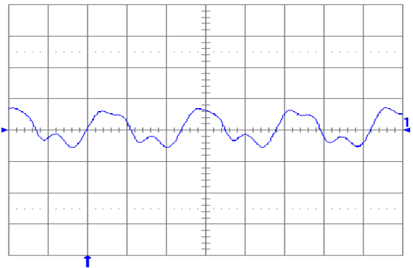
Figure 18. Output voltage ripple (20 mV/div.) at full rated load current into a resistive load with C_o = 10\text{ }\mu\text{F} tantalum + 1 \mu\text{F} ceramic and V_{in} = 48\text{ V} . Time scale: 1 s/div.
