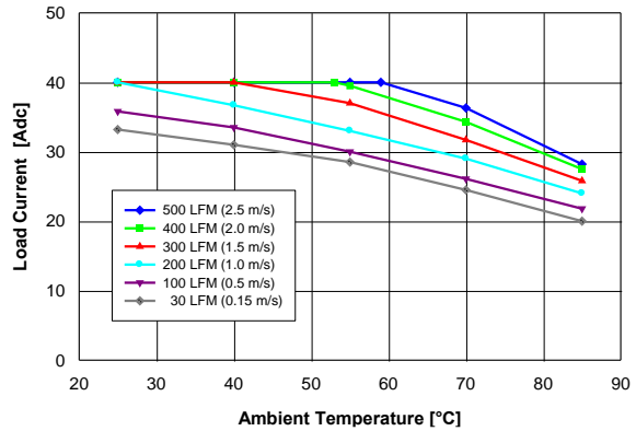
Figure 10. Available load current vs. ambient air temperature and airflow rates for QM48S40033 converter mounted horizontally with air flowing from pin 3 to pin 1, MOSFET temperature \leq 120 °C, V_{in} = 48 V.
