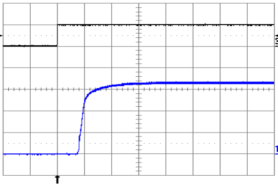
Figure 15. Turn-on transient at full rated load current (resistive) with no out-put capacitor at V_{in} = 48\text{ V} , triggered via ON/OFF pin. Top trace: ON/OFF signal (5 V/div.). Bottom trace: output voltage (1 V/div.) Time scale: 2 ms/div.
