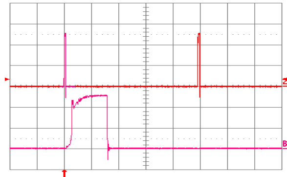
Figure 23. Load current (top trace, 20 A/div, 20 ms/div) into a 10 m \Omega short circuit during restart, at V_{in} = 48 V. Bottom trace (20 A/div, 1 ms/div) is an expansion of the on-time portion of the top trace.
