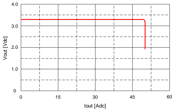
Figure 22. Output voltage vs. load current showing current limit point and converter shutdown point. Input voltage has almost no effect on current limit characteristic.
