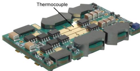
Figure 5. Location of the thermocouple for thermal testing.
