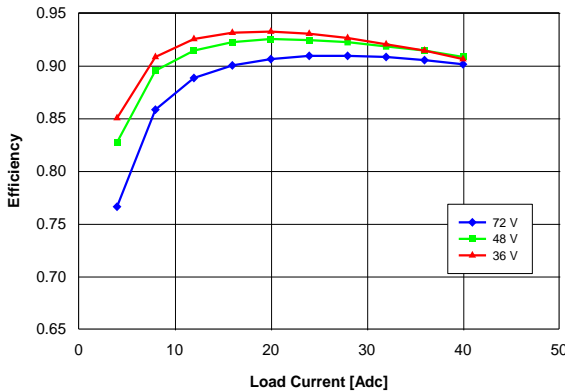
Figure 11. Efficiency vs. load current and input voltage for converter mounted vertically with air flowing from pin 3 to pin 1 at a rate of 300 LFM (1.5 m/s) and T_a = 25 °C.
