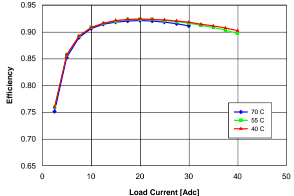
Figure 12. Efficiency vs. load current and ambient temperature for converter mounted vertically with V_{in} = 48 V and air flowing from pin 3 to pin 1 at a rate of 200 LFM (1.0 m/s).
