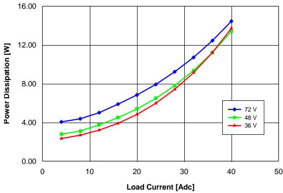
Figure 13. Power dissipation vs. load current and input voltage for converter mounted vertically with air flowing from pin 3 to pin 1 at a rate of 300 LFM (1.5 m/s) and T_a = 25^\circ\text{C} .
