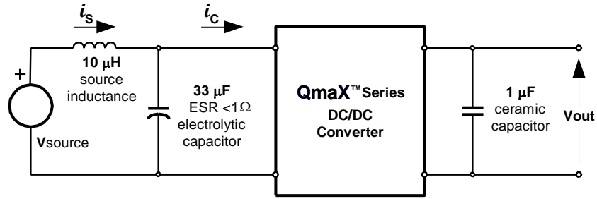
Figure 19. Test setup for measuring input reflected ripple currents, i_c and i_s .
