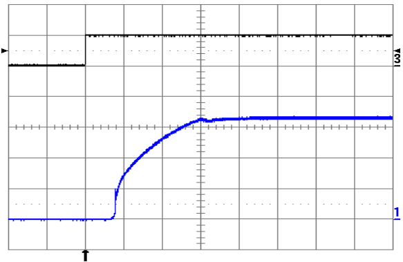
Figure 16. Turn-on transient at full rated load current (resistive) plus 40,000 \mu\text{F} at V_{in} = 48\text{ V} , triggered via ON/OFF pin. Top trace: ON/OFF signal (5 V/div.). Bottom trace: output voltage (1 V/div.). Time scale: 2 ms/div.
