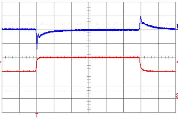
Figure 17. Output voltage response to load current step-change (20 A – 30 A – 20 A) at V_{in} = 48\text{ V} . Top trace: output voltage (100 mV/div.). Bottom trace: load current (10 A/div). Current slew rate: 1 A/ \mu\text{s} . C_o = 470\text{ }\mu\text{F} tantalum + 1 \mu\text{F} ceramic. Time scale: 0.2 ms/div.
