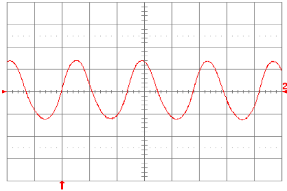
Figure 21. Input reflected ripple current, i_c (100 mA/div), measured at in-put terminals at full rated load current and V_{in} = 48 V. Refer to Fig. 19 for test setup. Time scale: 1 \mu s/div.
