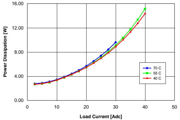
Figure 14. Power dissipation vs. load current and ambient temperature for converter mounted vertically with V_{in} = 48\text{ V} and air flowing from pin 3 to pin 1 at a rate of 200 LFM (1.0 m/s).
