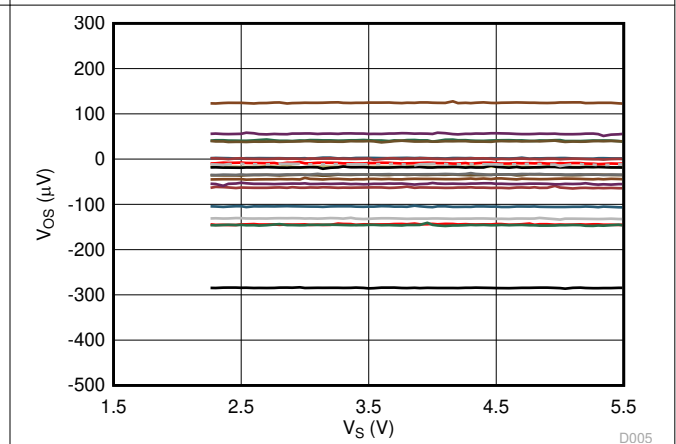
Figure 7-6. Offset Voltage vs Power Supply
