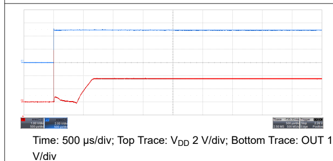
Figure 9-6. Output Turnon Response Time Without a Capacitive Load and V_{\text{DD}} = 5 \text{ V}
