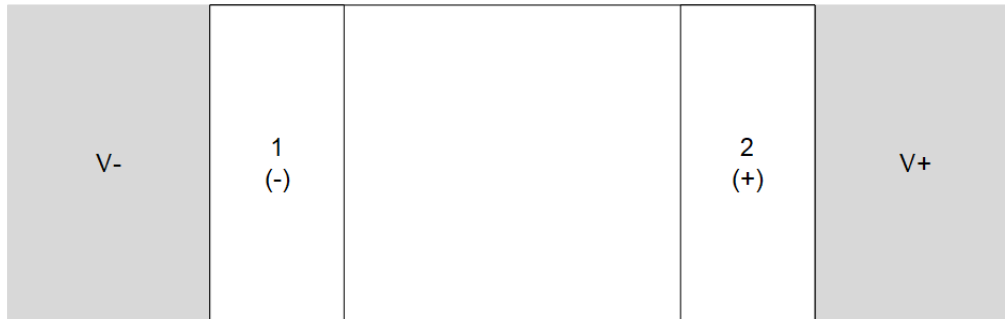
Figure 11-1. DEC Package Recommended Layout
