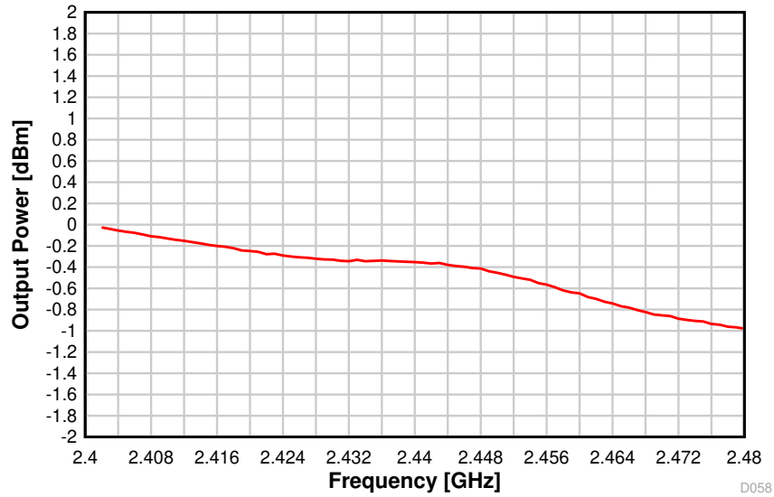
Figure 8-18. Output Power vs. Frequency (BLE 1 Mbps, 2.44 GHz)
