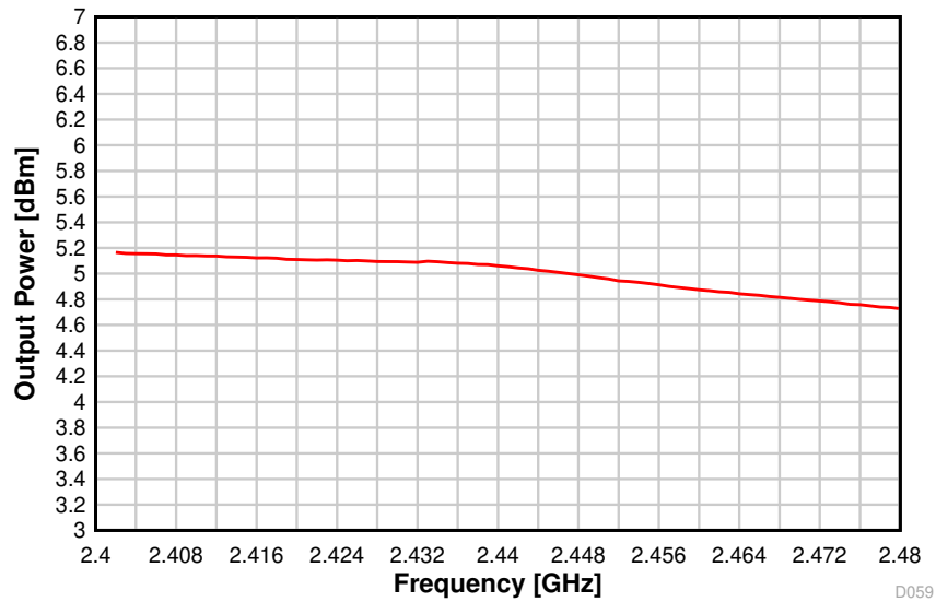
Figure 8-19. Output Power vs. Frequency (BLE 1 Mbps, 2.44 GHz, +5 dBm)
