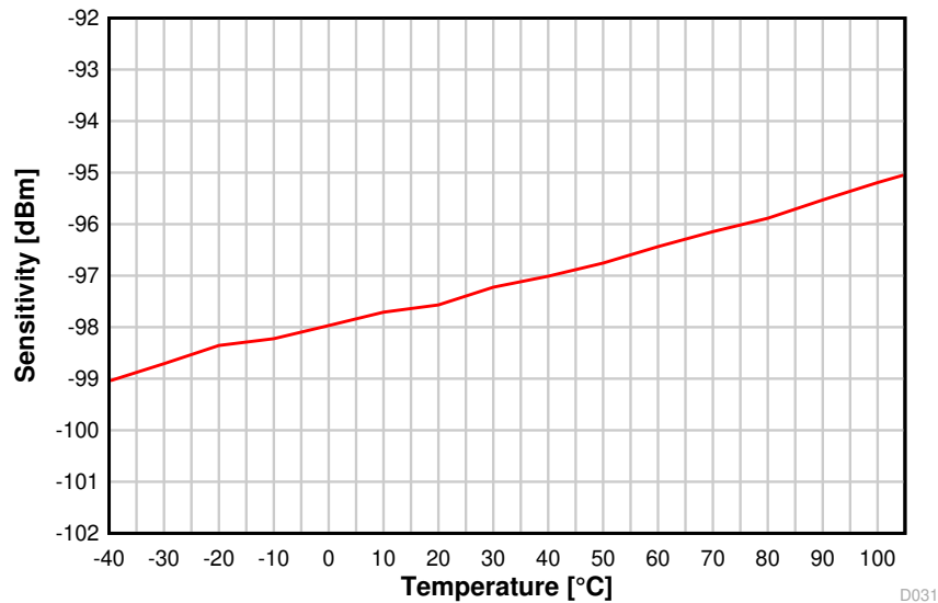
Figure 8-11. Sensitivity vs. Temperature (BLE 1 Mbps, 2.44 GHz)
